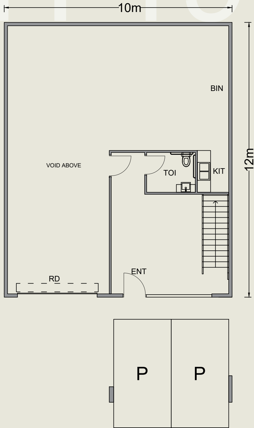
Ground Floor
