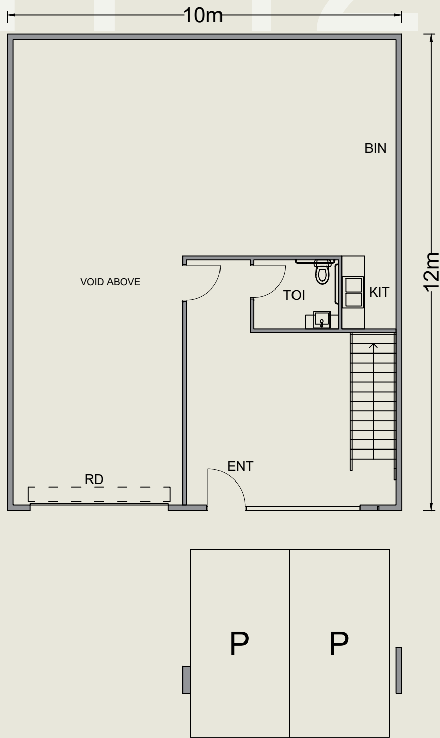
Ground Floor
