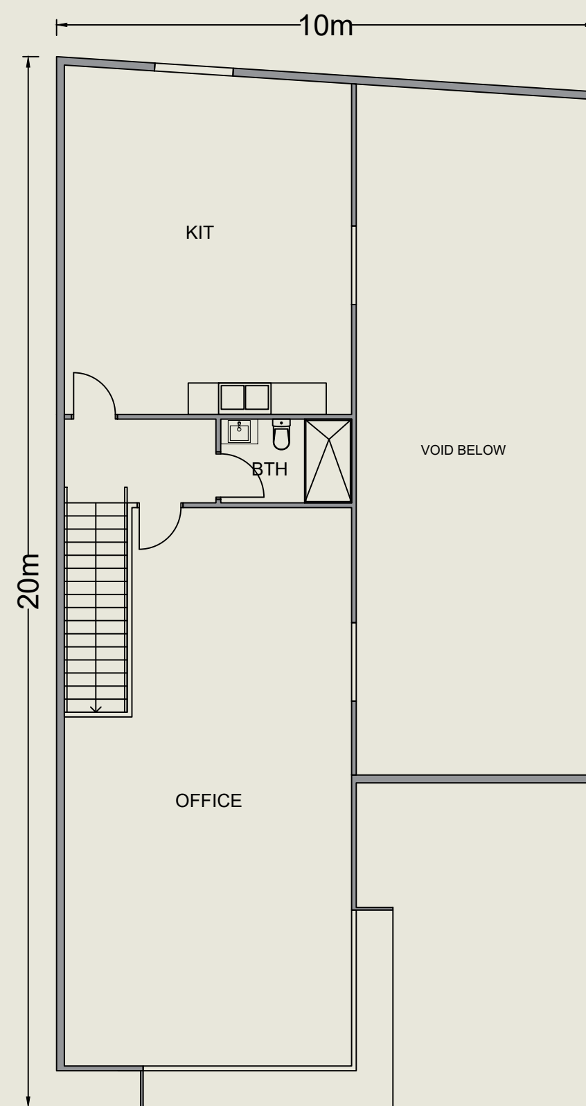
First Floor
