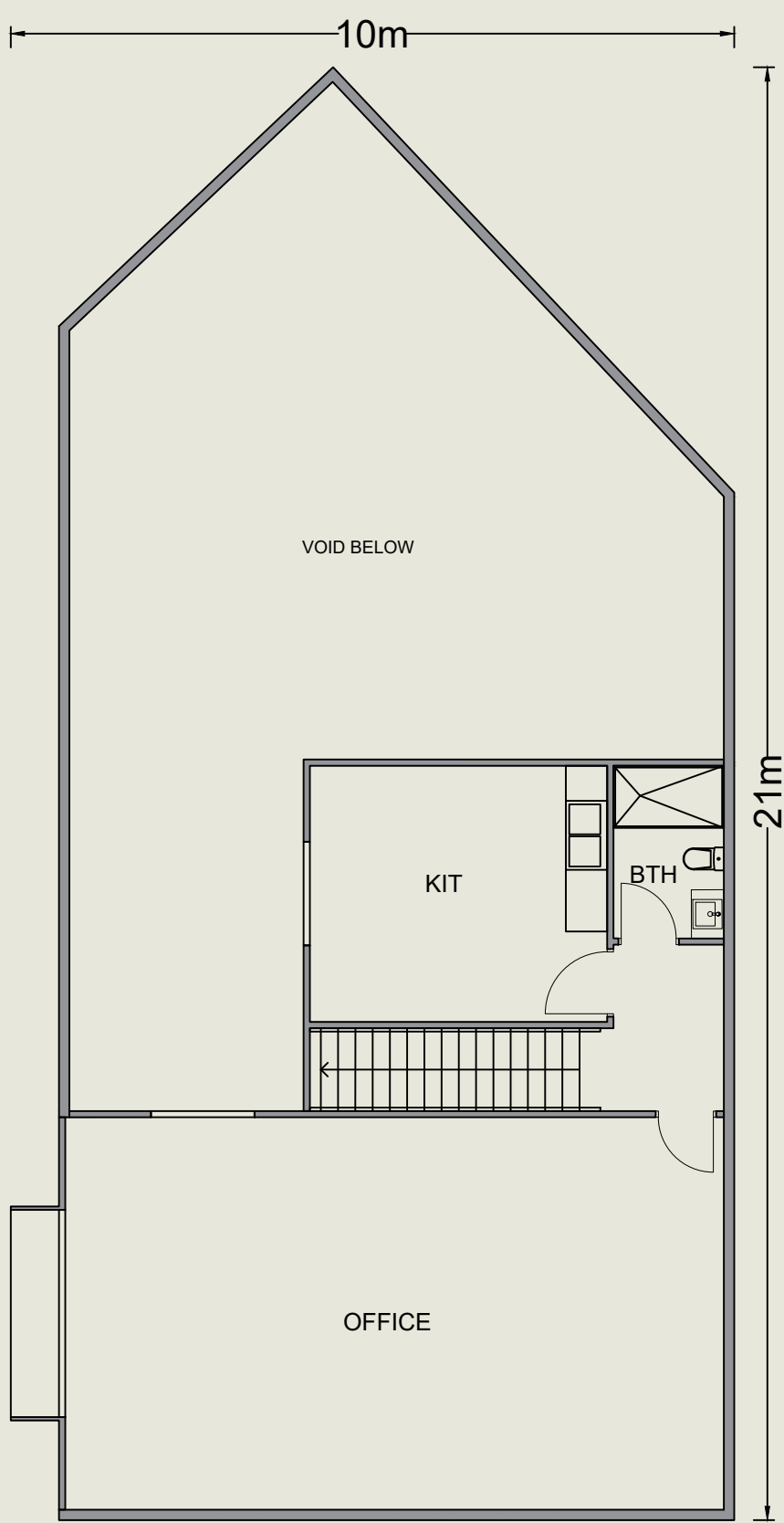
First Floor
