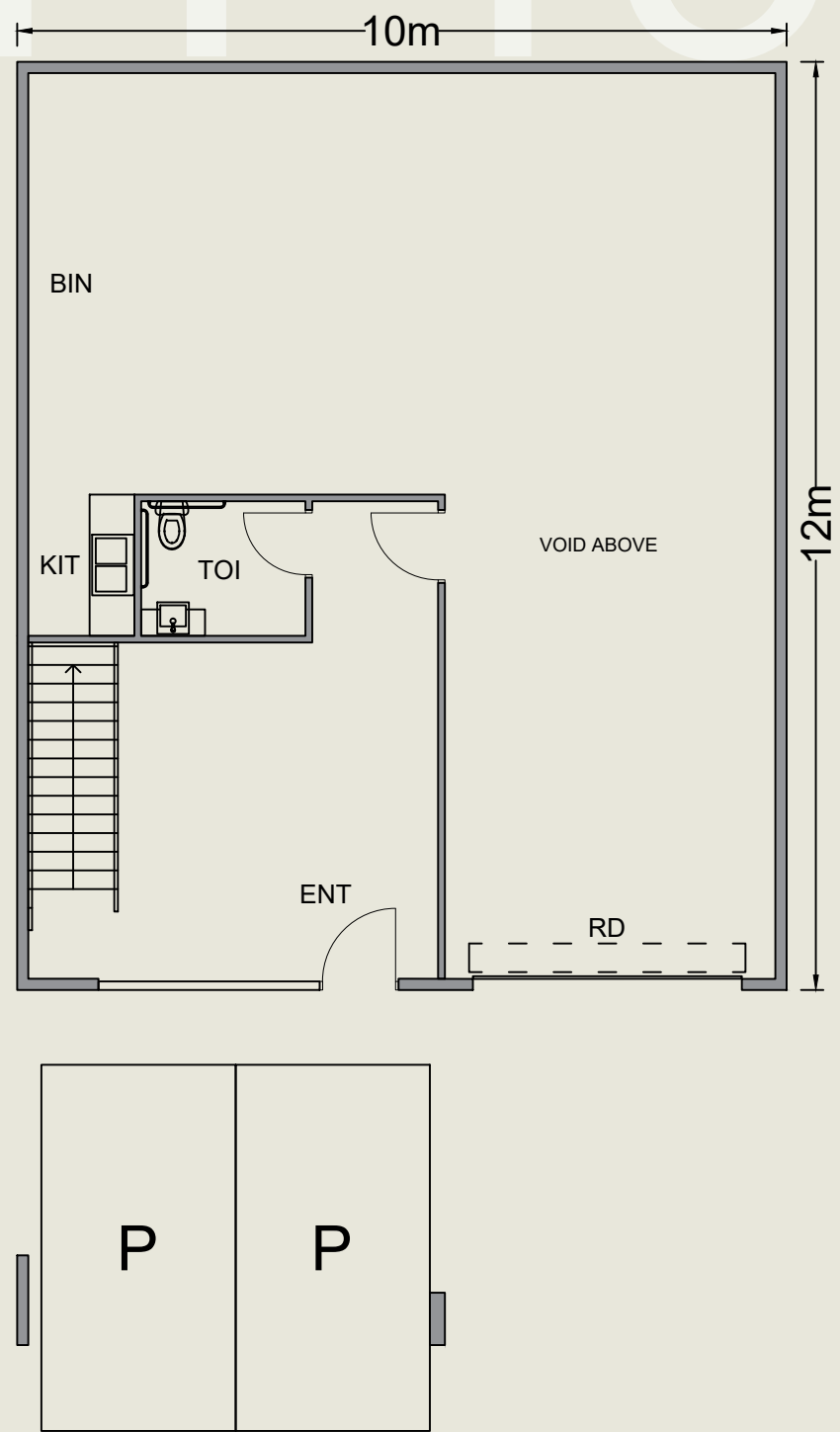
Ground Floor
